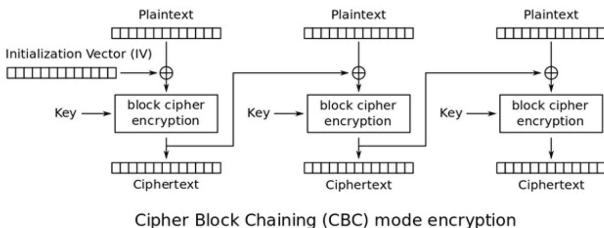
Figure 2: Diagram of the CBC mode of operation. Source: WhiteTimberwolf via Wikimedia Commons
